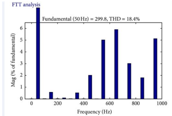
Figure.3.8 output voltage
