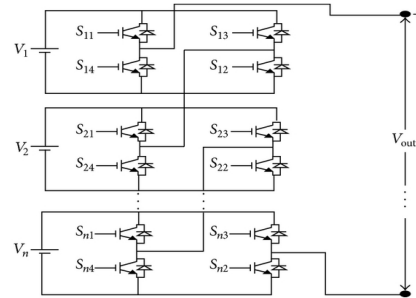
Fig 1.7-level,9-switch multilevel inverter
