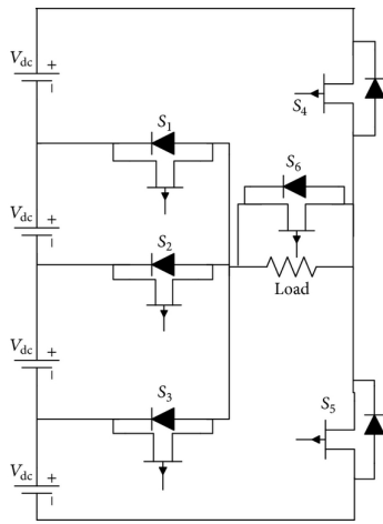
Fig 2.7-level,6-switch topology
