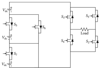
Fig.3 7-level,7-switch topology
