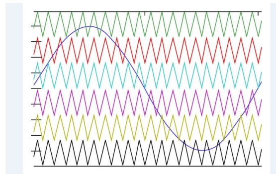
Fig;Carrier alignment of carrier based PWM techniqa
