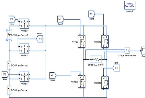
Fig 5; simulation diagram of proposed system
